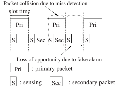
Fig. 2. Operation example of sensing based cognitive radios.
