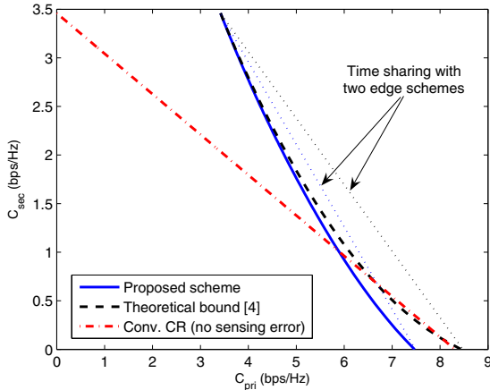
Fig. 7. Achievable rate region comparison when each link SNR is given by h_1 = 15\text{dB} , h_2 = 20\text{dB} , h_3 = 15\text{dB} , h_4 = 15\text{dB} and h_5 = 10\text{dB} .
