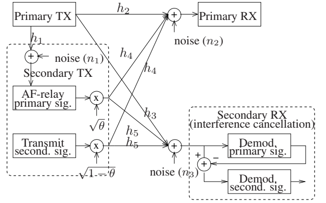
Fig. 5. Proposed transmission scheme for cognitive radios.
